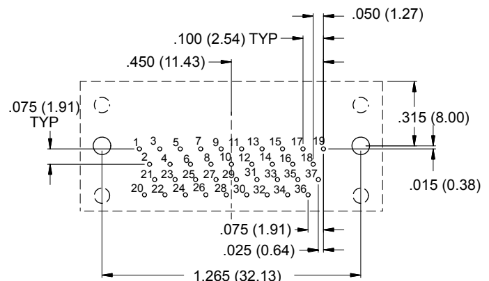
37 PIN
