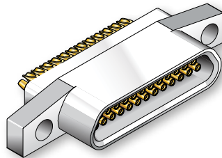
Figure 4 Socket (Receptacle) with Thru-Hole Mounting (B) .096/.088 Dia. (2.43/2.23)
