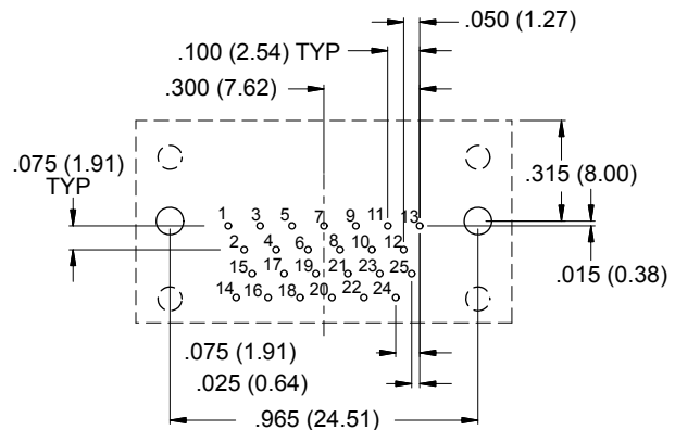
25 PIN
