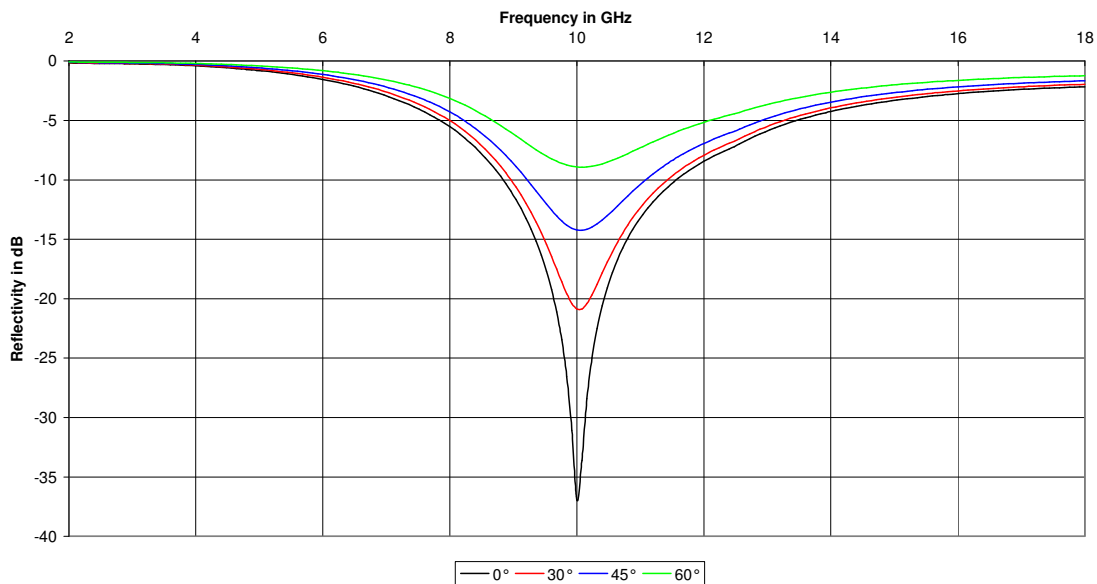
Typical reflectivity at various angles of incidence ECCOSORB DSF-U-10 Perpendicular polarization
