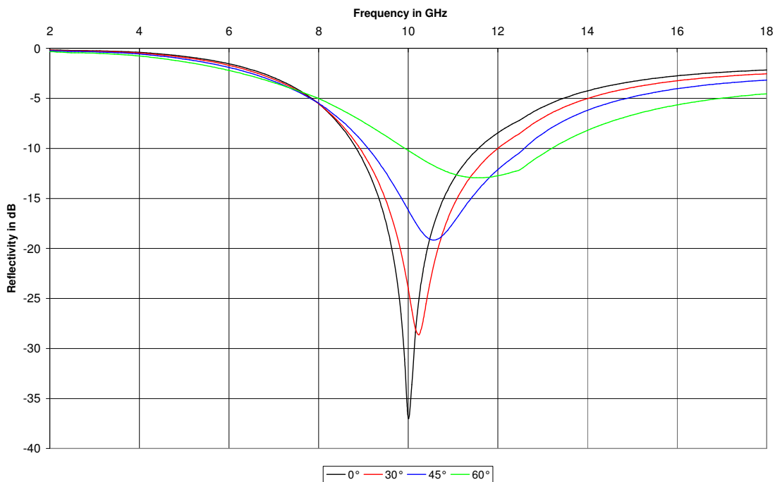
Typical reflectivity at various angles of incidence ECCOSORB DSF-U-10 Parallel polarization
